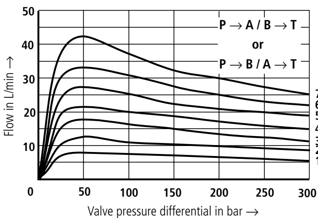
Performance limit, nominal flow 30 L/min
